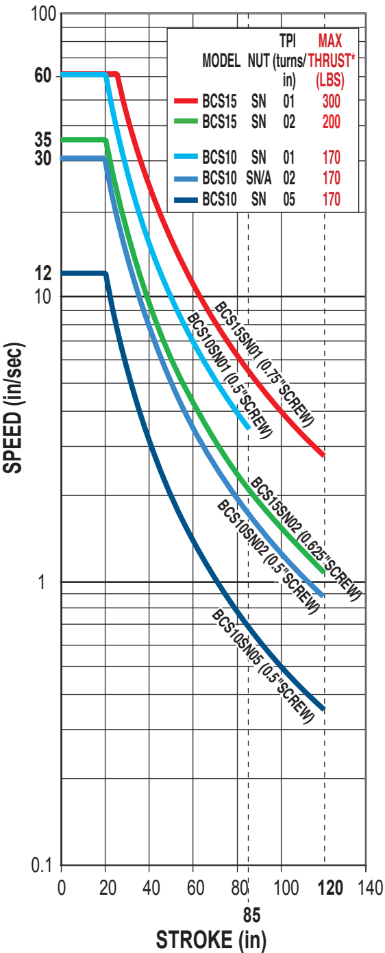
CRITICAL SPEED WITH US CONVENTIONAL ACME SCREW
